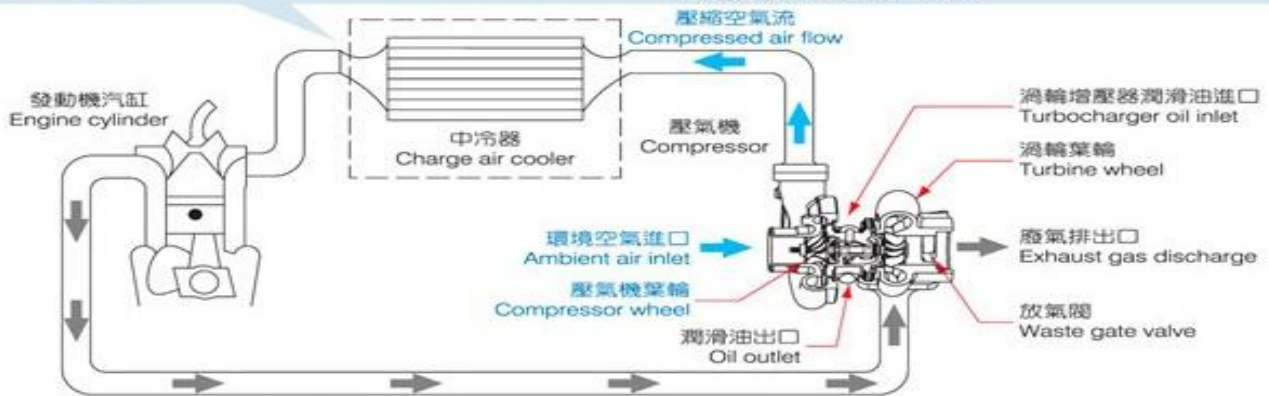
渦輪增壓器工作原理圖 - Illustration of Turbocharger Operating Principle
